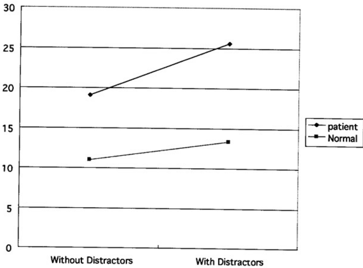
FIG. 6. Comparison of navigation index between WOD and WD in both groups.
